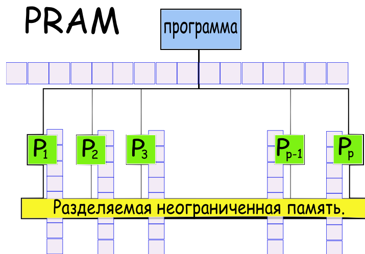
Рис. 4.3: PRAM — Parallel Random Access Machine
